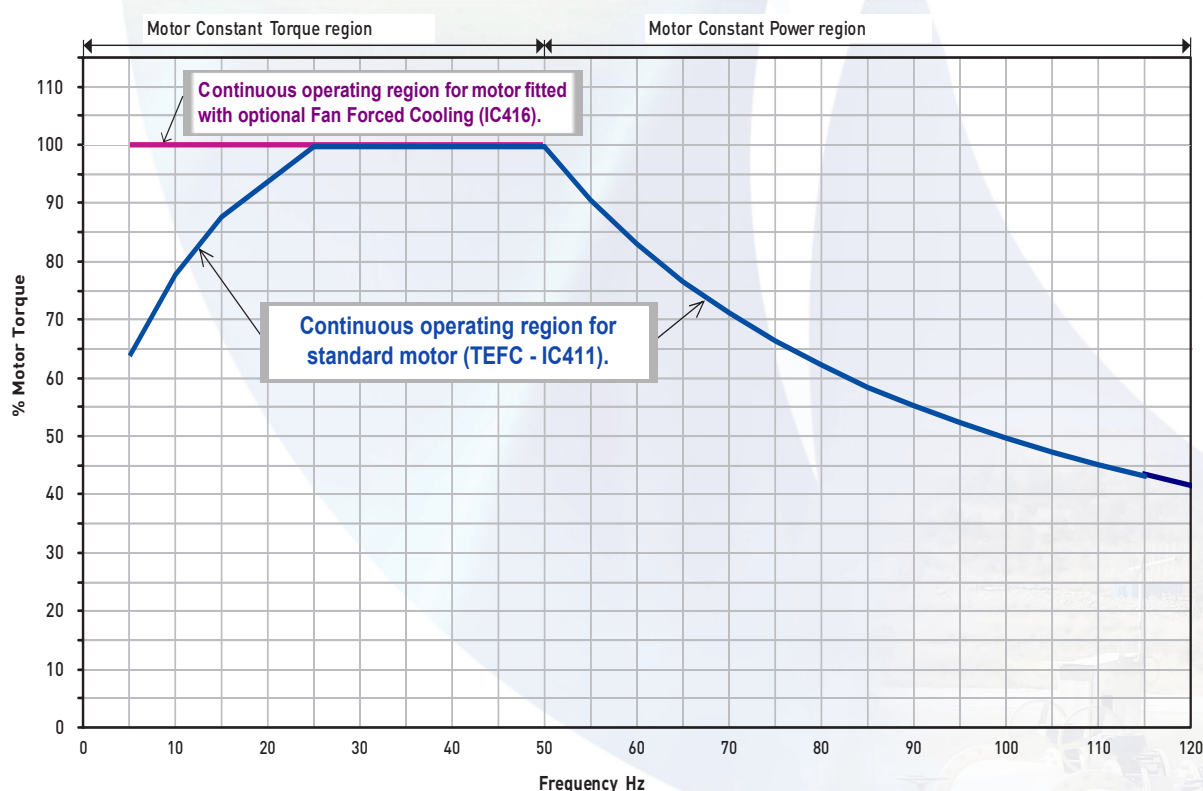
Typical Motor Loadability Curves For VSD Duty
