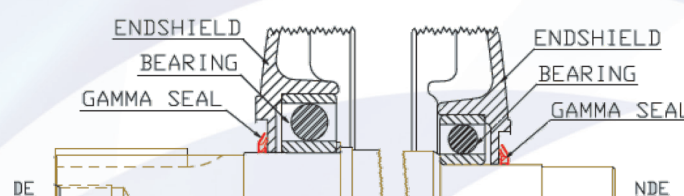
SEVERE DUTY BEARING ARRANGEMENT WITH GAMMA SEALS
