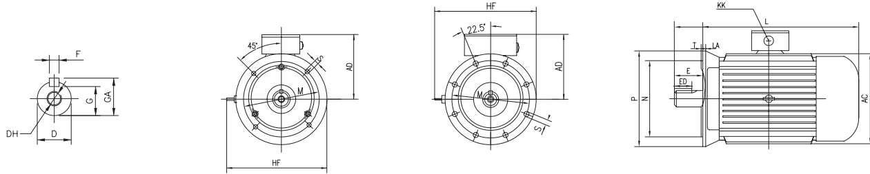
SHAFT DETAIL
